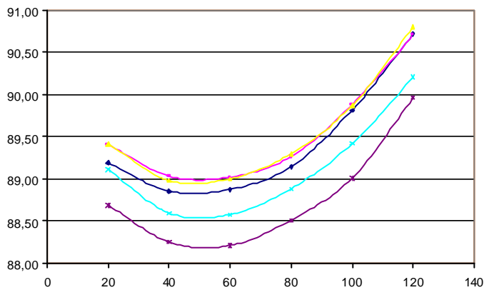
Figure 2.3 Sensitivity temperature drift (@1 MHz , 5V)
