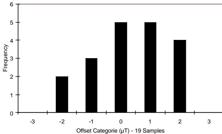
Figure 2.4 Offset distribution( \mu T ) (@1 MHz , 5V)
