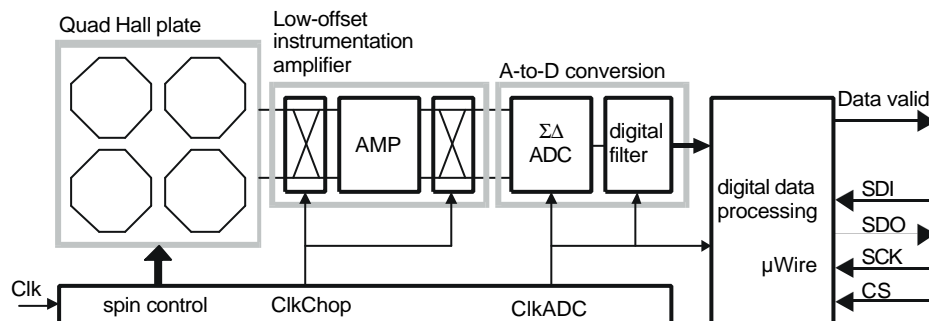
Figure 1.1 XEN-1200 scheme with Quad Hall plate sensor
